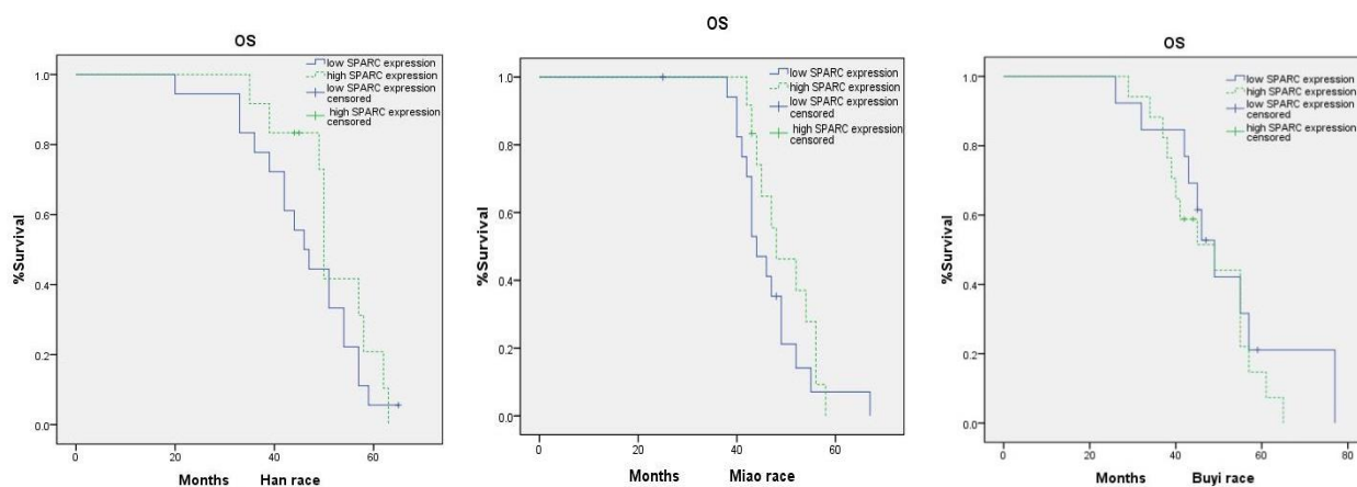
Figure 2. Kaplan-Meier estimates for OS by high expression group and low expression group in Han, Miao and Buyi race.
