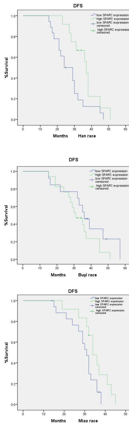
Figure 1. Kaplan–Meier estimates for DFS by high expression group and low expression group in Han, Miao and Buyi race.
